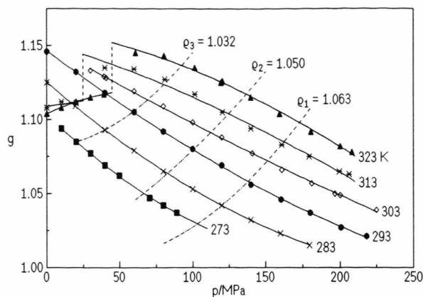
Fig. 4. Kirkwood- g -factor for TBN as a function of pressure for different temperatures and densities (in \text{g/cm}^3 ).
